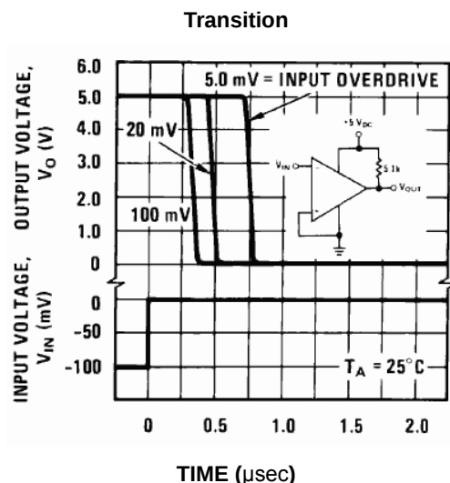
Response Time for Various Input Overdrives—Negative
