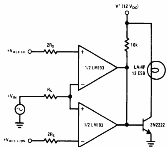
Limit Comparator
