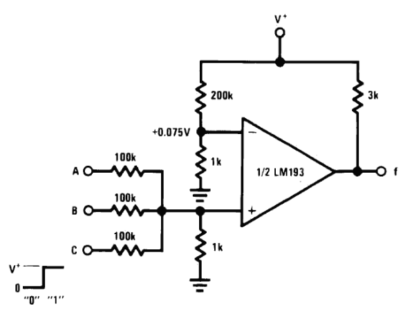
OR Gate
