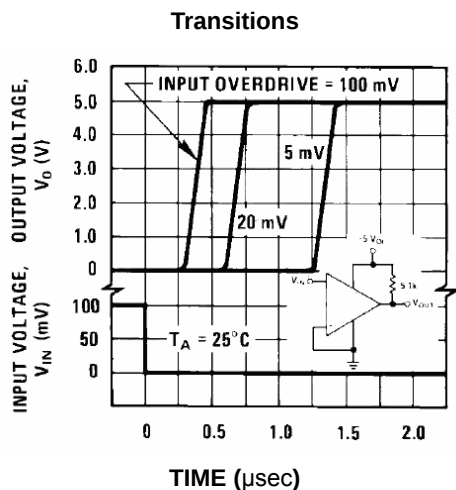
Response Time for Various Input Overdrives —Positive Transitions
