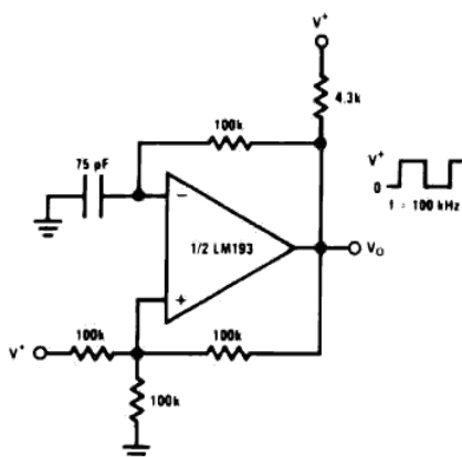
Squarewave Oscillator
