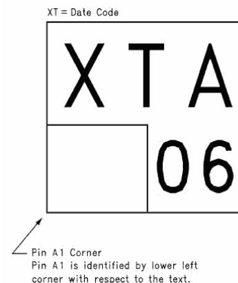
micro SMD Marking
