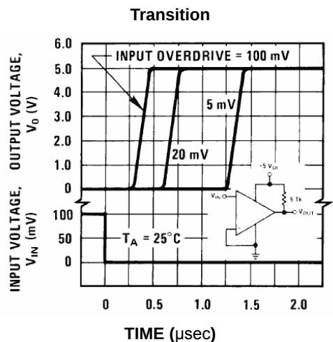
Response Time for Various Input Overdrives—Positive
